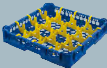
Cestello bicchieri a 16 scomparti (113x113 mm) Glass rack with 16 compartments (113x113 mm)
