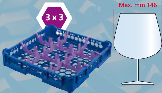
Cestello 50x50 cm con griglia viola - 9 scomparti 50x50 cm rack with purple divider insert - 9 compartments
